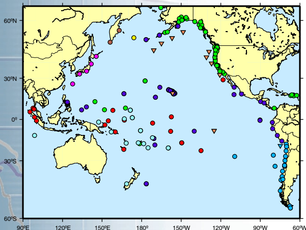
Sea level network used by PTWC to monitor Pacific sea levels. Circles show coastal sea level stations and triangles show NOAA DART systems. Colors indicate responsible agency: PTWC (dark blue), NOAA National Ocean Service (green), Univ of Hawaii Sea Level Center (red), SHOA (blue green), JMA (pink), Russian Hydromet (brown), Australia National Tidal Center (light blue), WC/ATWC (yellow), NOAA National Data Buoy Center (orange).
