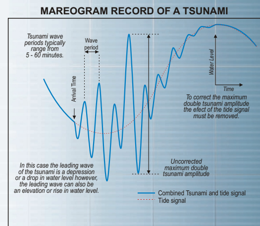
Mareogram (sea level) record of a tsunami.
