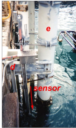
Rarotonga sea level station, Avarua Harbor, Cook Islands. The fiberglass electronics package (a), antenna (b), solar panel (c) were installed on a pier. Conduit (d) containing cables connecting the sensor, located at a depth of five feet below low-tide water level, to the data collection platform containing the electronics above, was externally attached to the tube containing the sensor (e).
