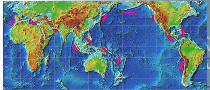
Global tsunami source zones. Tsunami hazards exist in all oceans and basins, but occur most frequently in the Pacific Ocean. Tsunamis can occur anywhere and at any time because earthquakes cannot be accurately predicted.
