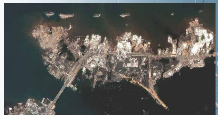
Banda Aceh, Sumatra, Indonesia. The tsunami of 26 December 2004 completely razed coastal towns and villages, leaving behind only sand, mud, and water where once there had been thriving communities of homes, offices, and green space.
