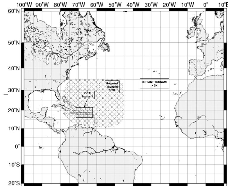
Figure 4. Schematic of areas for which tsunami warnings (Local or regional, less than 2 hours) or watches (distant, greater than 2 hours) would be issued.
