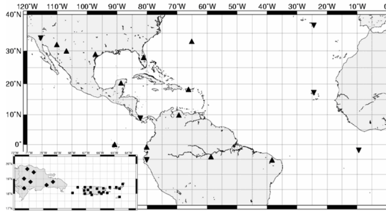
Figure 2. Seismic stations used by the Early Bird System running in the Puerto Rico Seismic Network for the detection of potentially tsunamigenic earthquakes. The insert corresponds to stations of the Puerto Rico Seismic Network (squares) and the “Instituto Sismológico Universitario” (ISU) of the Autonomous University of Santo Domingo (UASD) in the Dominican Republic. Stations of the IRIS/IDA (inverted triangles) and IRIS/USGS (triangles) networks are also used.
